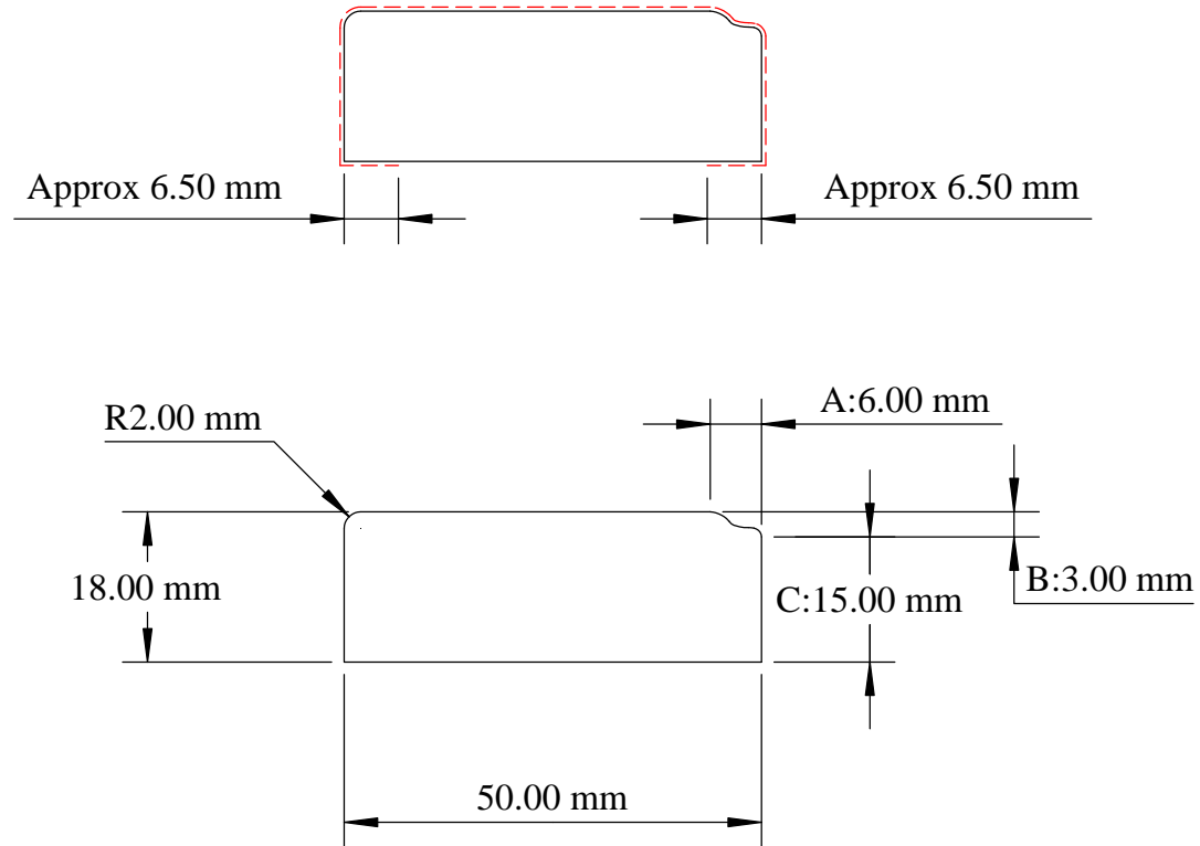
DRAWING FOR LOCATION OF WRAP. LENGTH OF WRAP 96mm.
